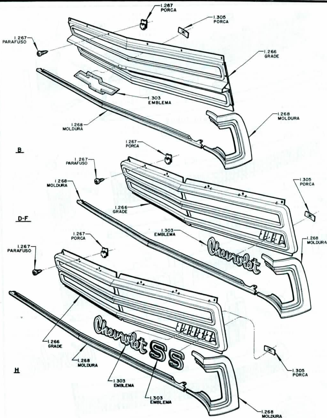
GRADE - RADIADOR - 1973/74
