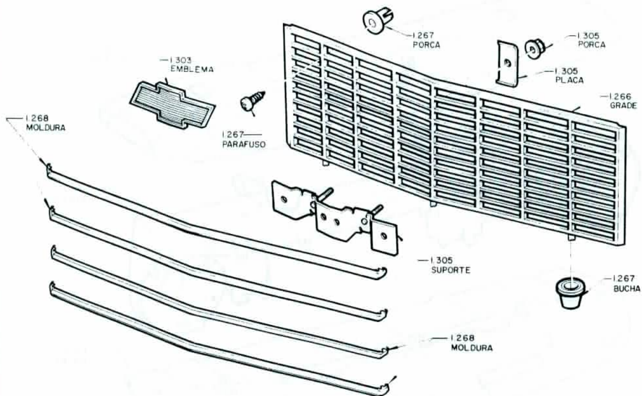
GRADE - RADIADOR - 1975/1977
